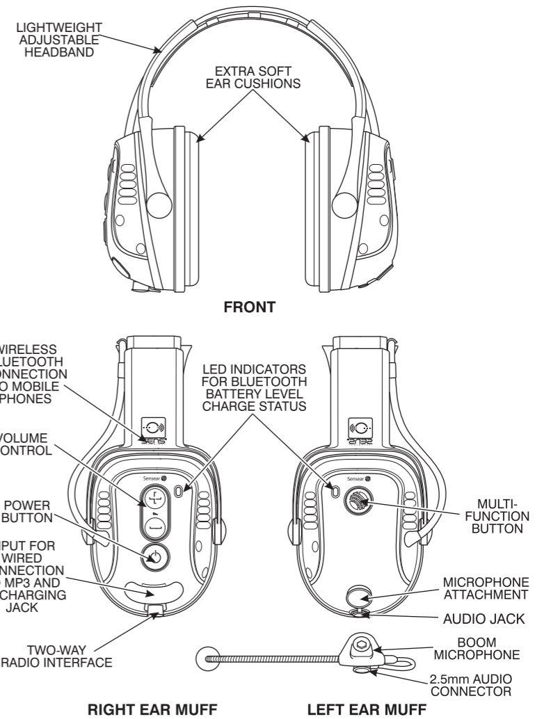
Figure 1: Sensear SM1/SM1x Major Components
